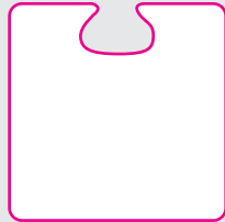
Nose Die (Sh8pe) 95mm x 95mm
